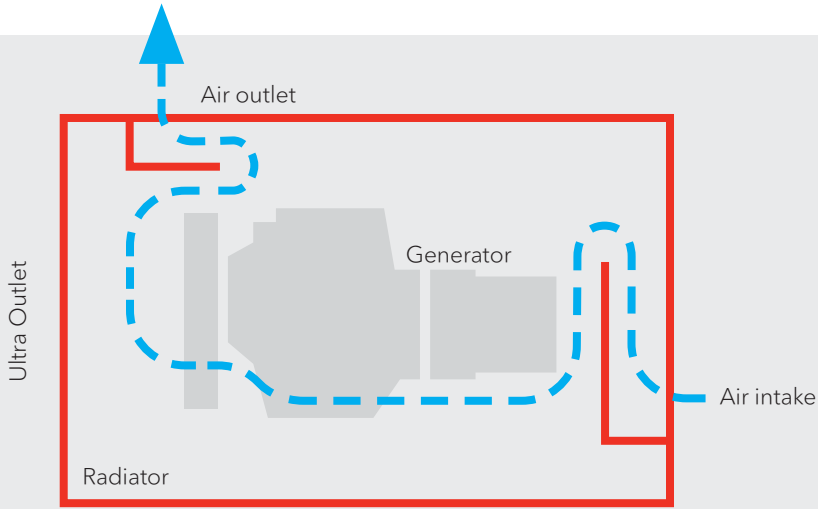
GS-PTY Series. In our 20 and 50kVA units, redirected cooling air doubles length of travel - lowering sound level dramatically.
